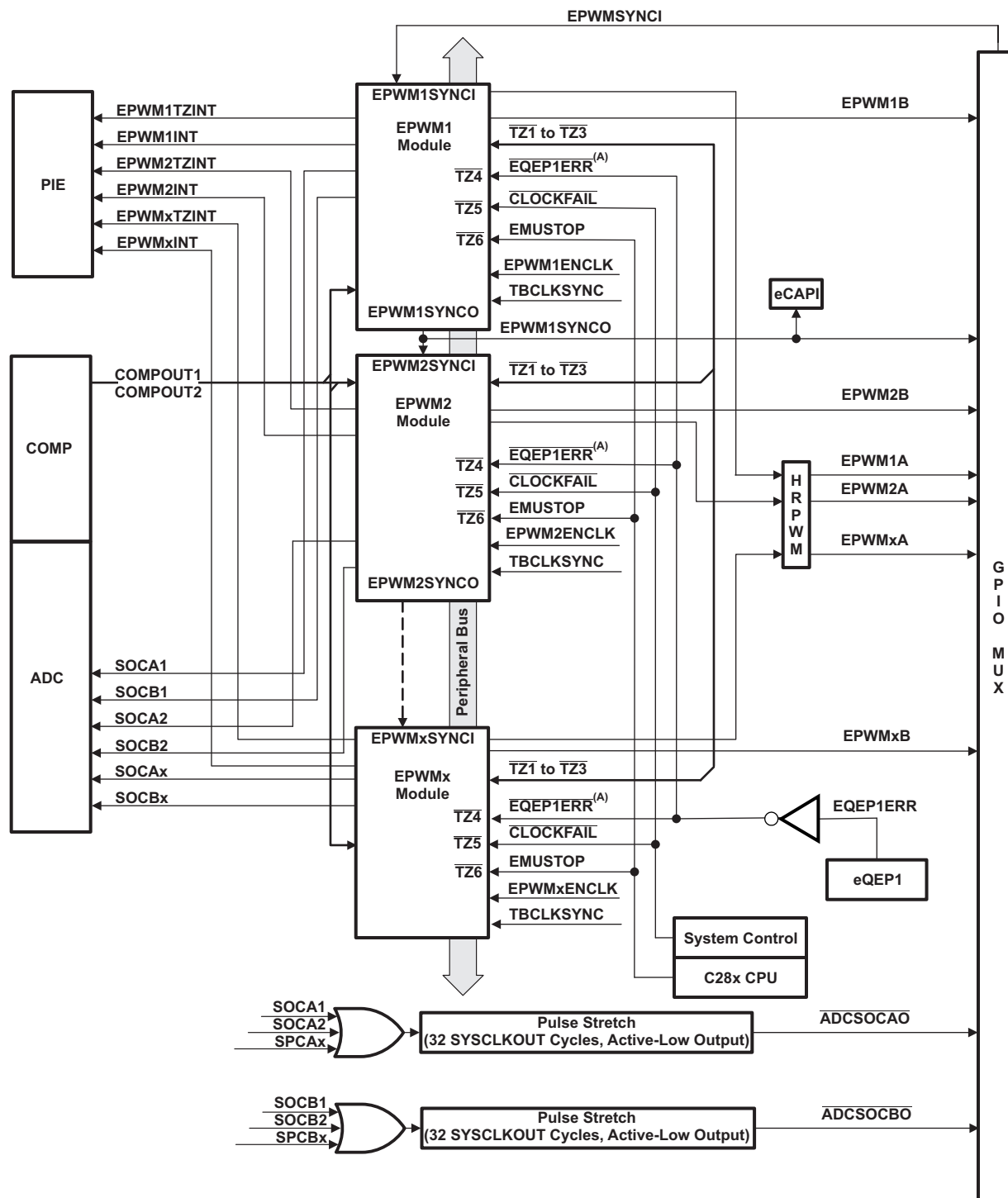
Figure 6-38. ePWM
