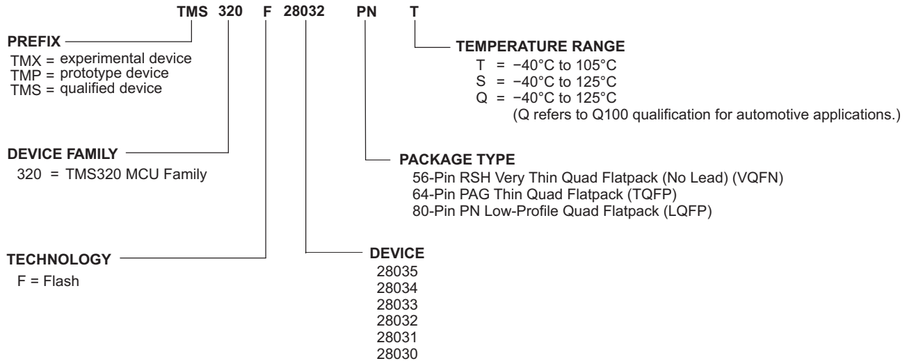
Figure 8-1. Device Nomenclature
